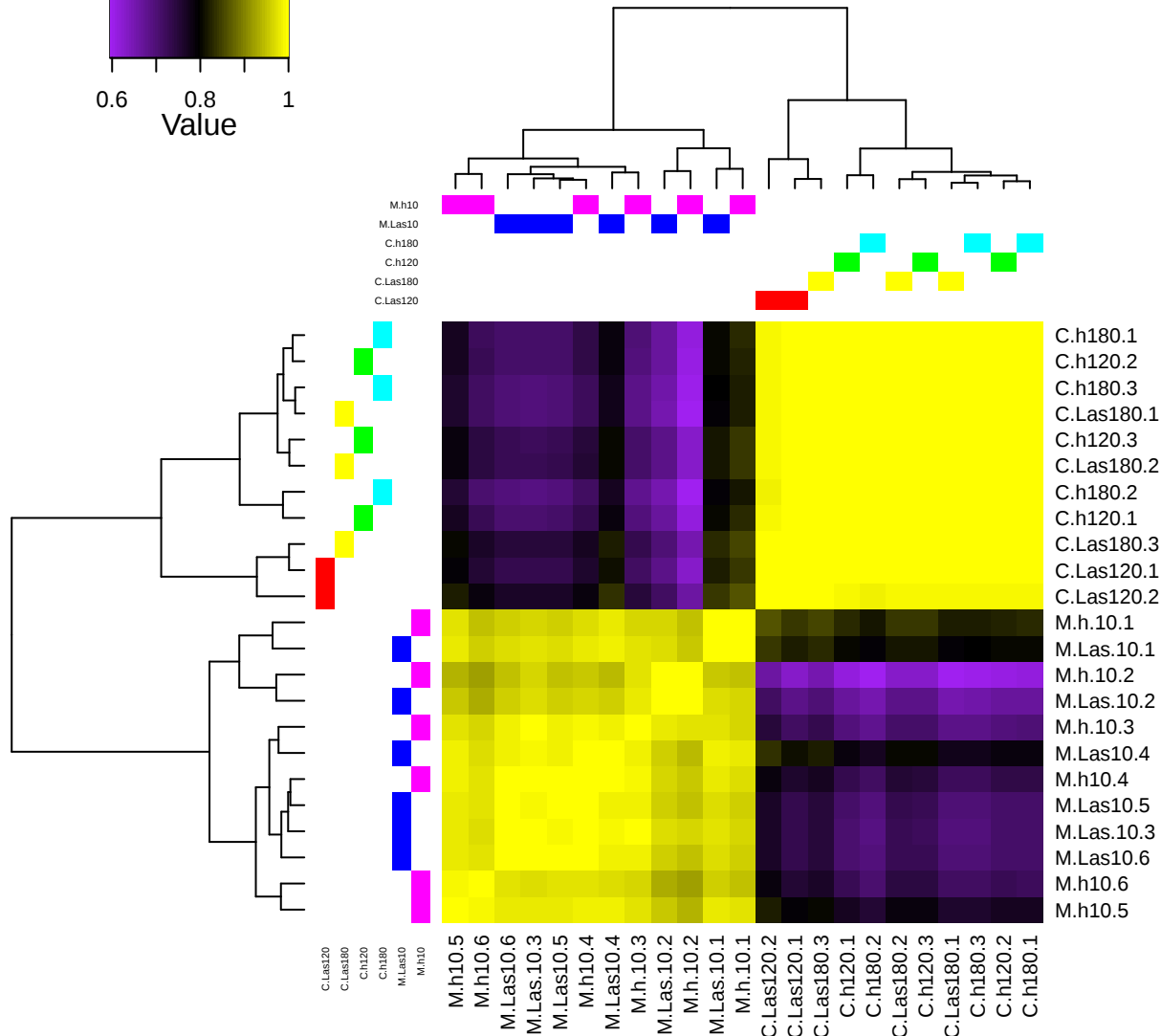
sample correlation matrix all.counts.revstranded.tsv.TPMs.tsv
