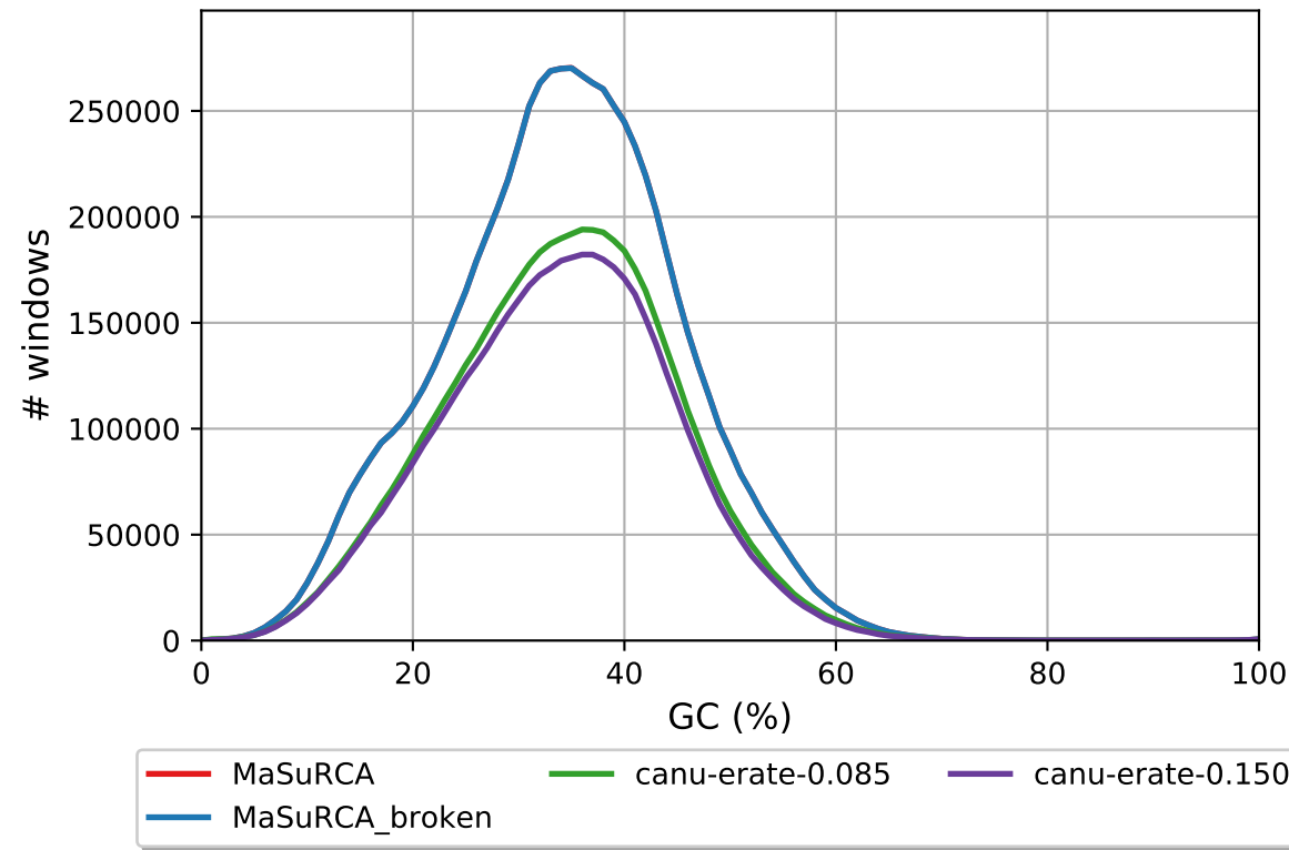
GC content
